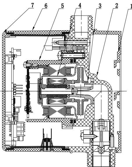
Fig. 7 Sectional drawing
