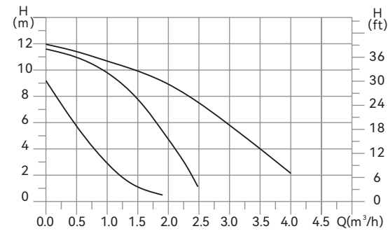
Basic 25-12S
