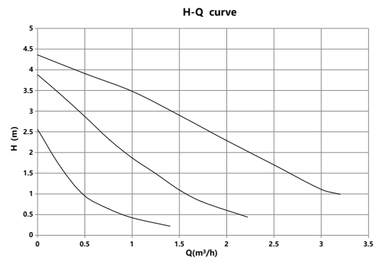
Basic 20-5S-130
