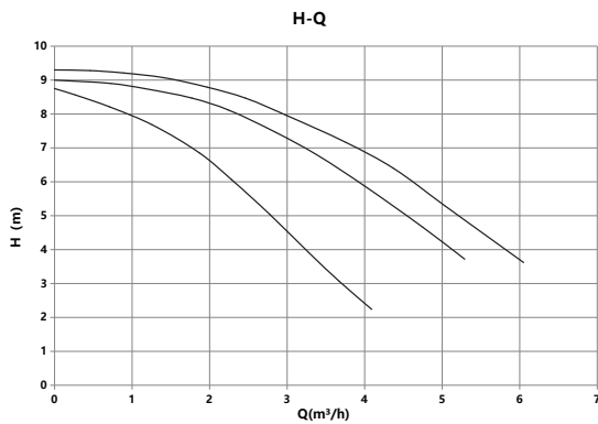
Basic 25-9S
