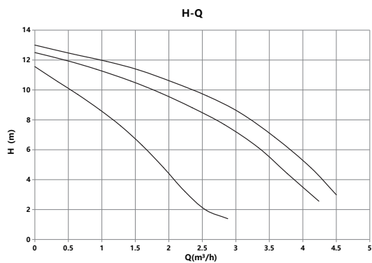
Basic 20-12SZ
