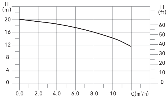
Basic 32-9SF
