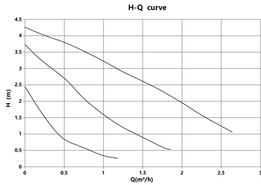
Basic 32-4S-180
