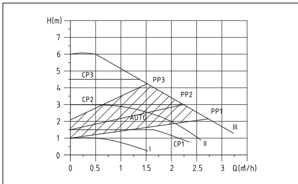
Master SD 20/25/32-6 180
