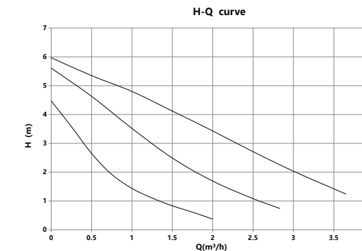
Basic 25-6S-130
