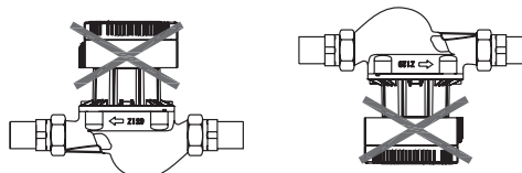
Fig. 34 Unacceptable position of the pump shaft
