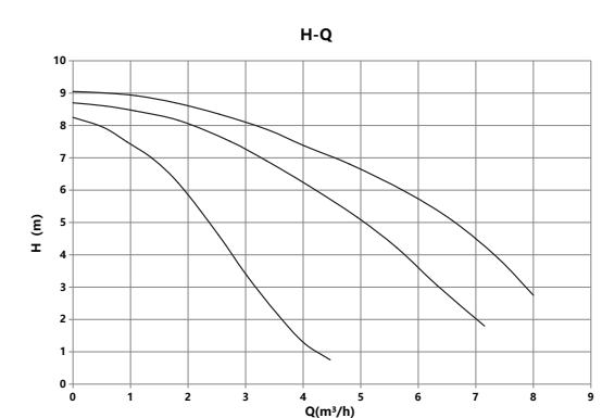
Basic 32-9S
