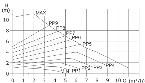
Fig. 38 Proportional-pressure curve settings
