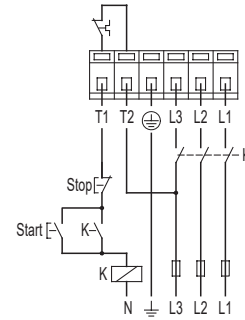
Fig. 20 Three-phase with a neutral wire
