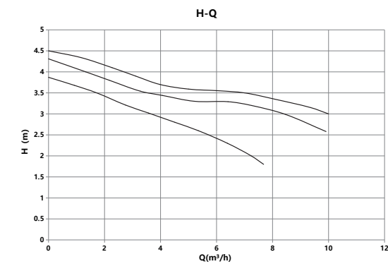
Basic 40-4.5SF
