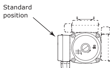
Fig. 9 The following position of the control box of the heating system
