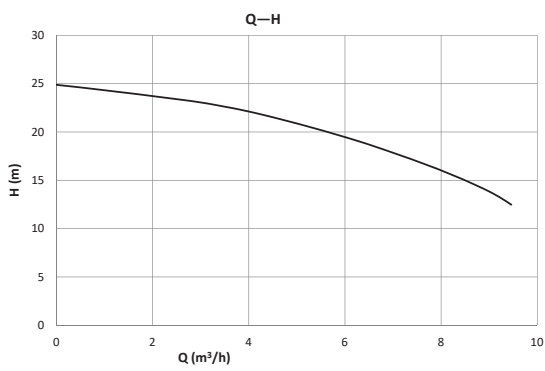
Basic 20-26Z
