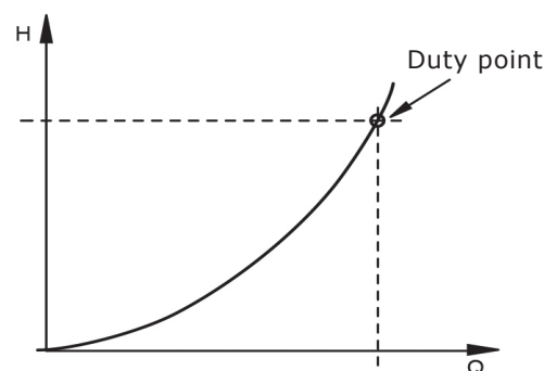
Fig. 1 System characteristic
