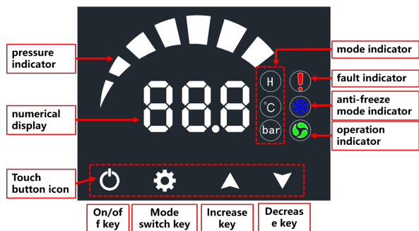
Fig.5 Operation interface
