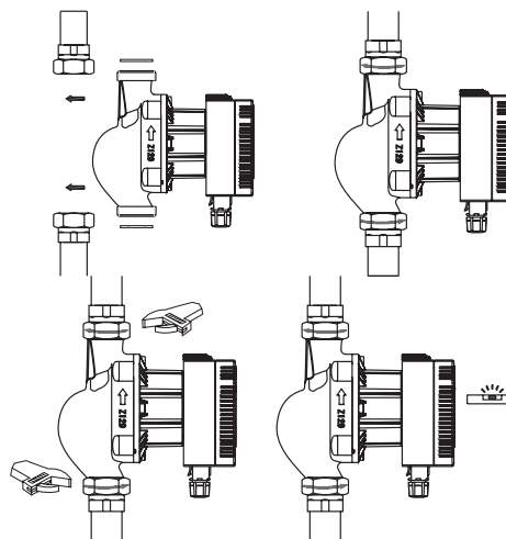
Fig. 35 Pump installation
