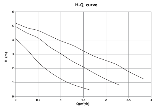
Basic 32-5S-180
