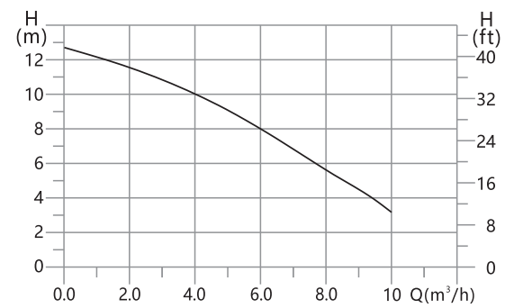
Basic 32-12SF
