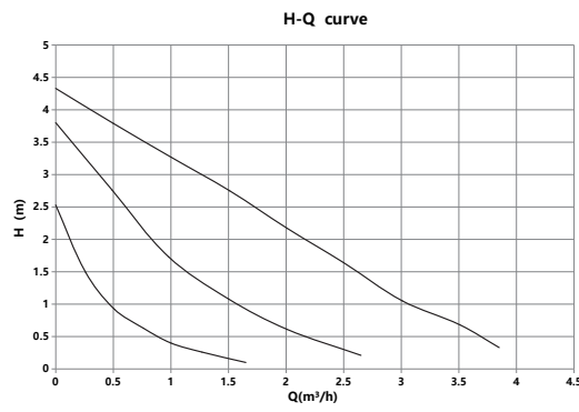
Basic 25-5S-130
