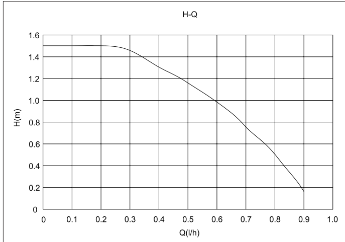
Fig.4 Performance curve
