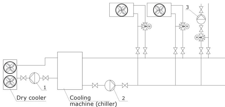
Fig. 32 Functional drawing of air conditioning system
