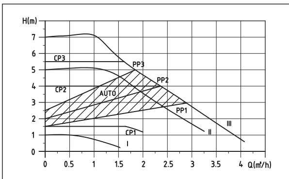
Master SD 20/25/32-7 180
