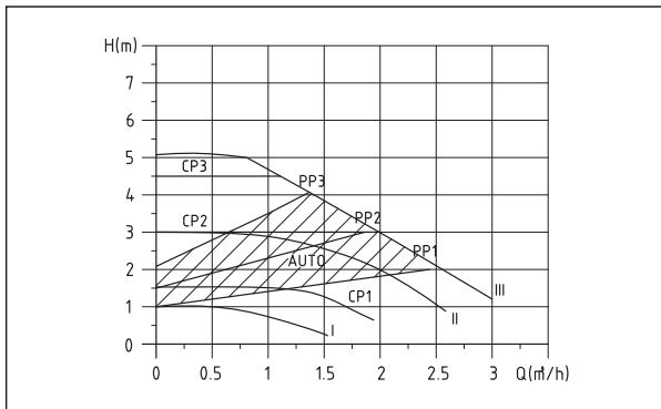
Master SD 20/25/32-5 180
