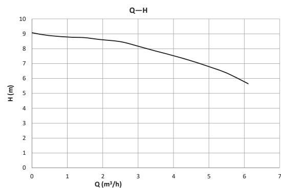
Basic 25-9Z
