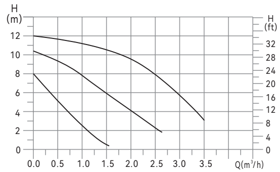
Basic 15-12S
