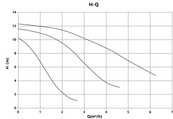
Basic 25-12SL
