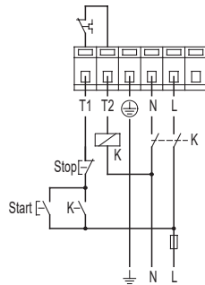
Fig. 18 Single phase
