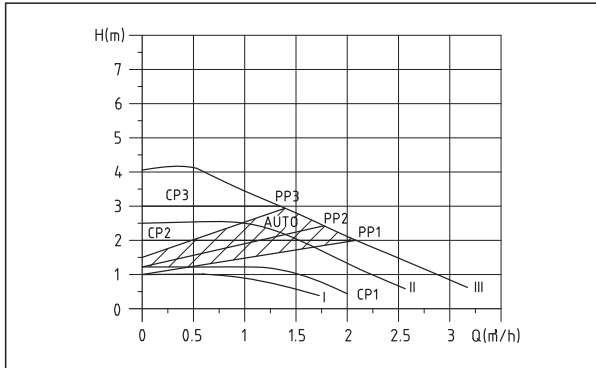
Master SD 20/25/32-4 180
