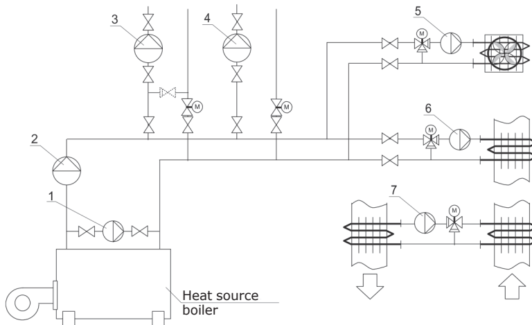
Fig. 31 Functional drawing of heating system
