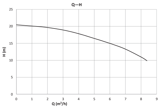
Basic 20-20Z
